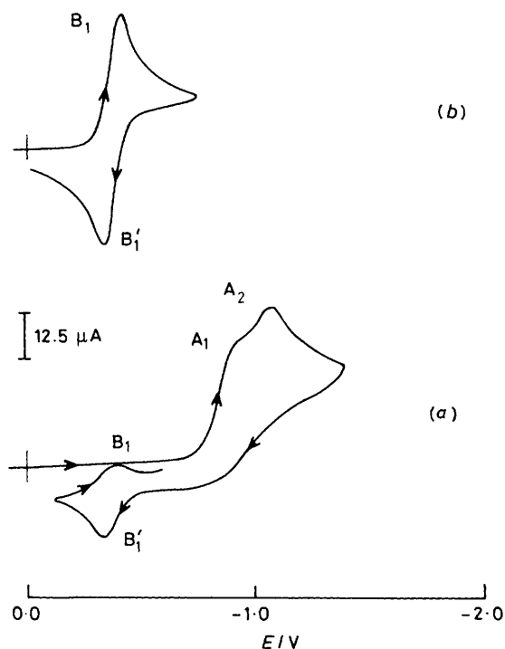
Figure 4. Cyclic voltammograms for (a) [\text{Fe}(\text{salen})(\text{ox})]^- and (b) [\text{Fe}(\text{salen})]^+ . Scan rate 100 \text{ mV s}^{-1} and 0.2 \text{ mol dm}^{-3} [\text{NBu}_4][\text{PF}_6]
